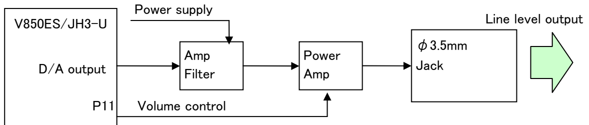
Audio output block diagram
